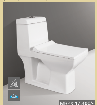
Di SPAN (P & S Trap) 670 x 360 x 725mm (S Trap - 100/225/300mm)
